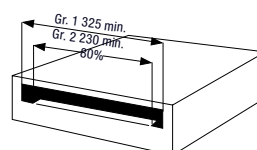
diagonal boxes type C
